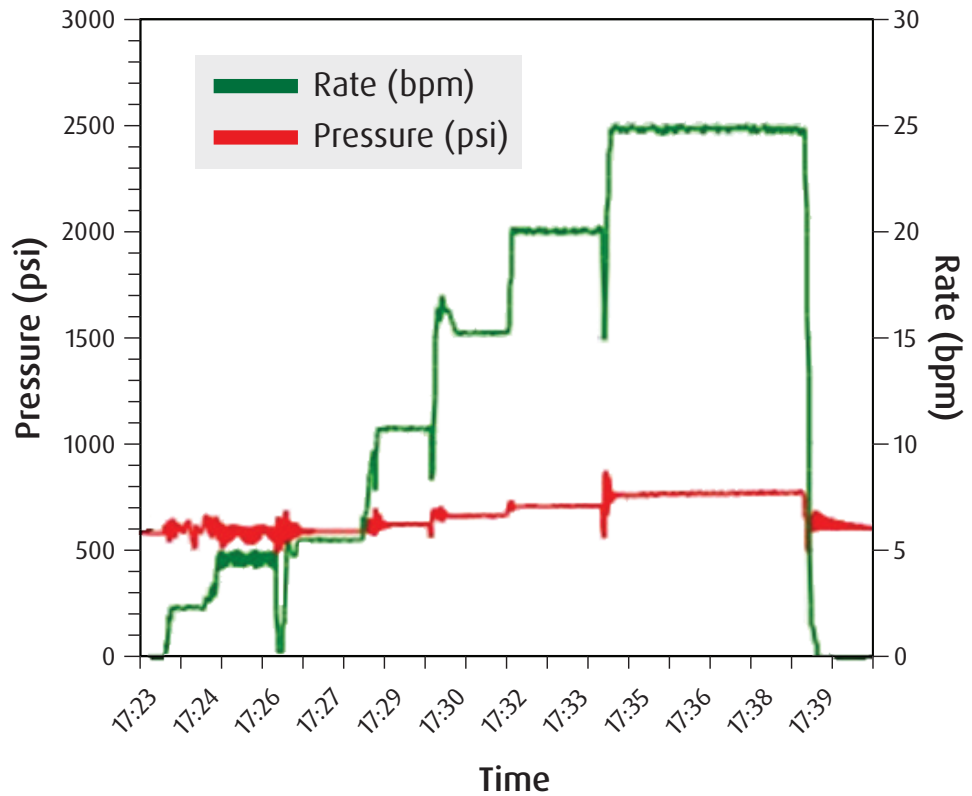
Delaware SWD Step-rate Test Results
